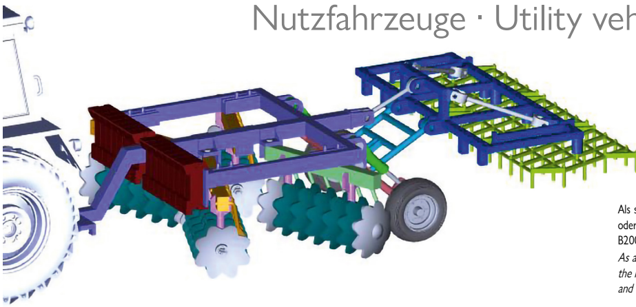
Set Pflug "Fortschritt B200" + Egge "Fortschritt B402" (GDR) Set plow "Fortschritt B200" + harrow "Fortschritt B402" (GDR)
